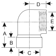
90° Adapter Elbow
