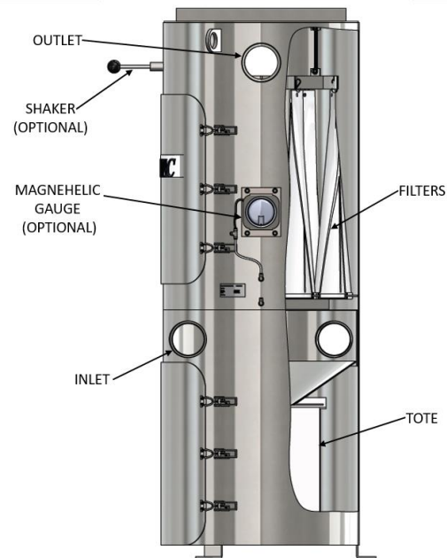
Eurovac III Double Pump System 10HP - 75HP (x 2) Turbine Vacuum Producers and Bag Filter Separators
